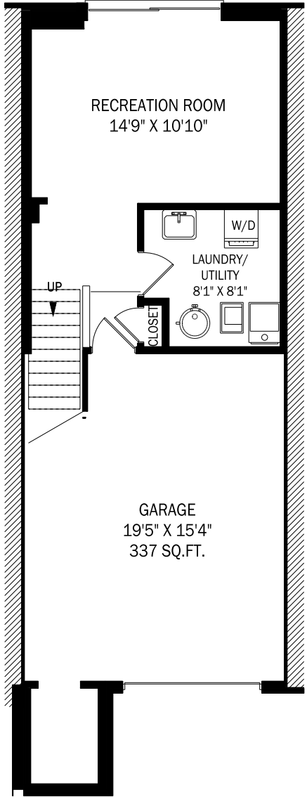
LOWER LEVEL - 341 SQUARE FEET
