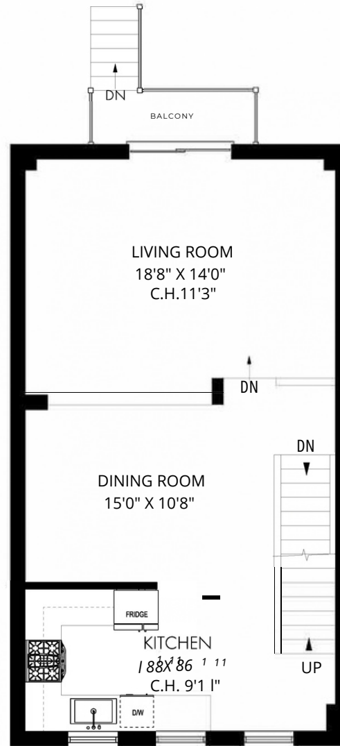
MAIN LEVEL -737 SQUARE FEET
